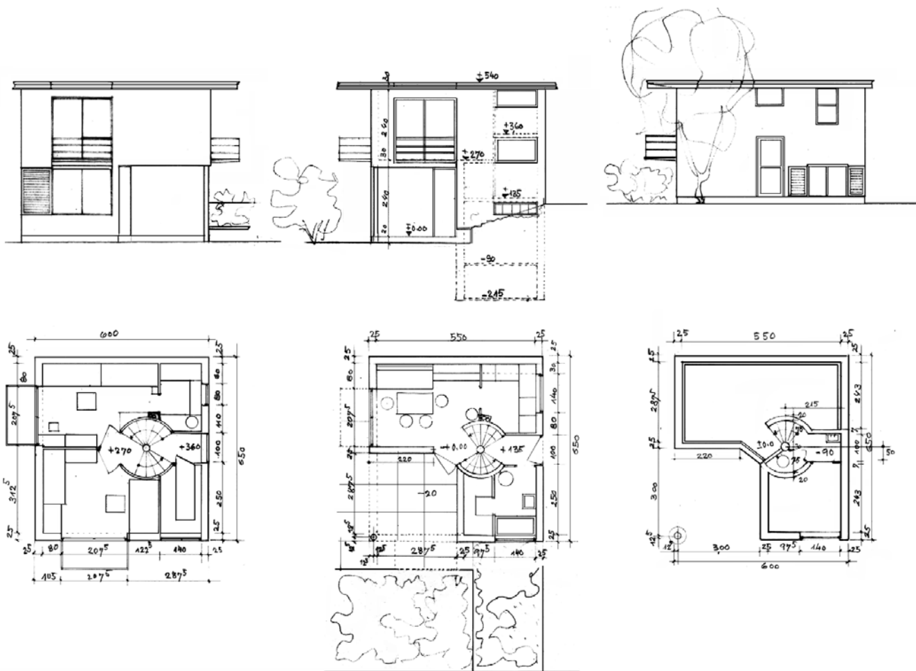
Vikendica Sekol, projekt / Sekol weekend house, project, Samobor, Jagnjić dol bb, 1969.
