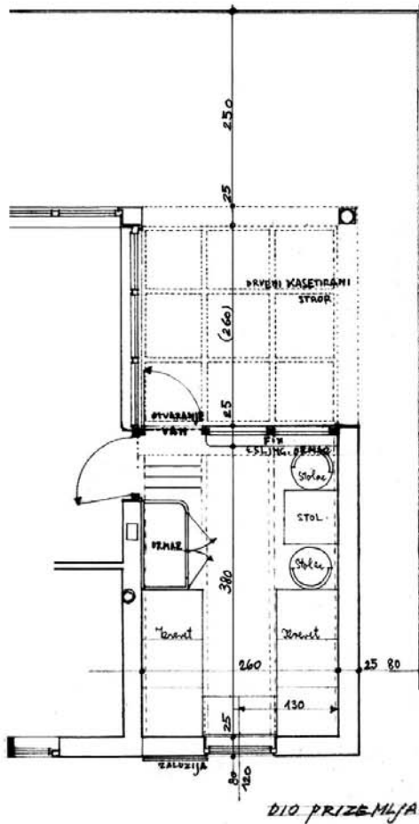
Klijet Damaška, nacrti / Damaška vineyard cottage, blueprints, Varaždin Breg, Dugi vrh 1940.
