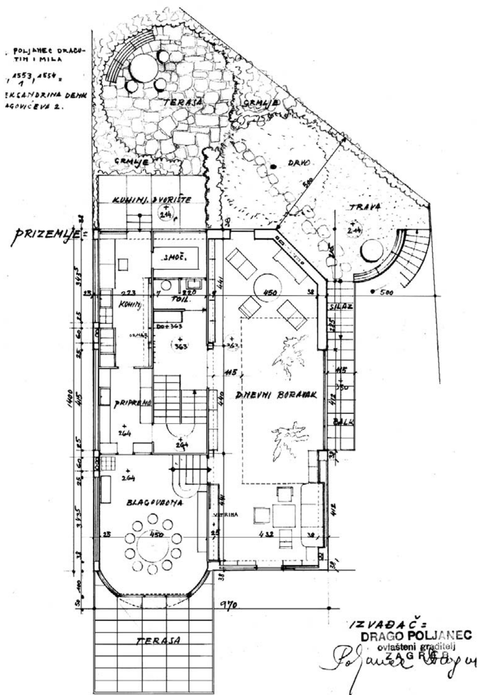
Vila Poljanec, tlocrt / Poljanec villa, ground plan , Zagreb, Alagovićeva 4, 1941-42.
